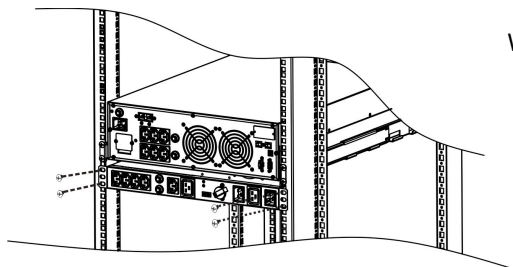
Chart 1: Rack mounting
