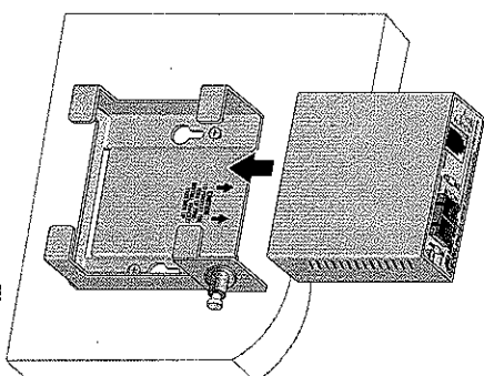
Figure 3. Sliding the Media Converter into the AT-WLMT-010 Bracket
