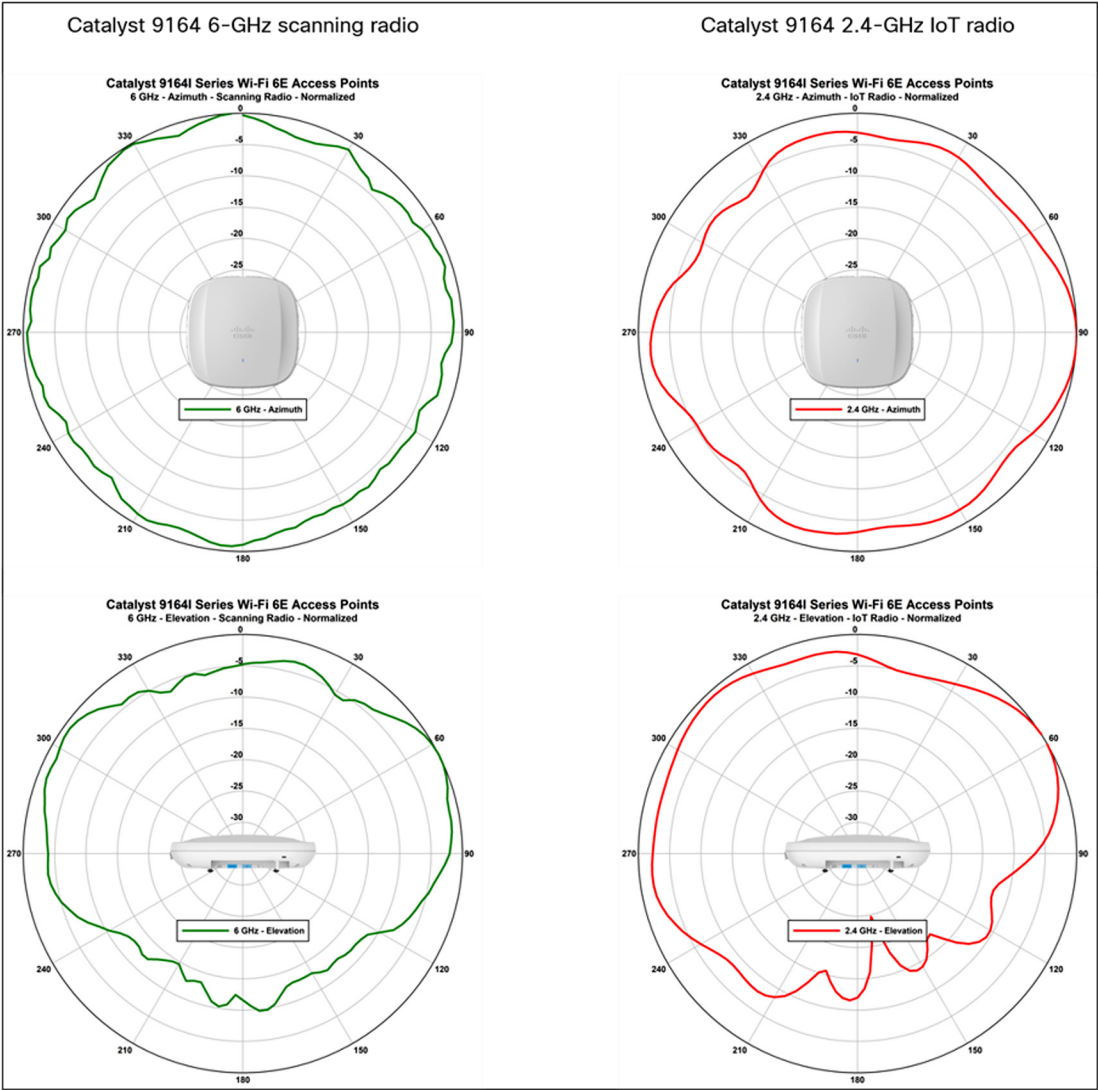
Figure 2. Antenna profiles
