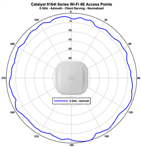
Catalyst 9164 5-GHz client serving radio
