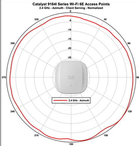
Catalyst 9164 2.4-GHz client serving radio
