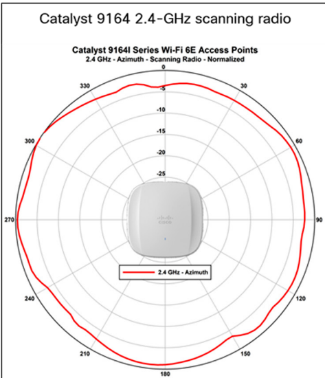
Catalyst 9164 Series Wi-Fi 6E Access Points
