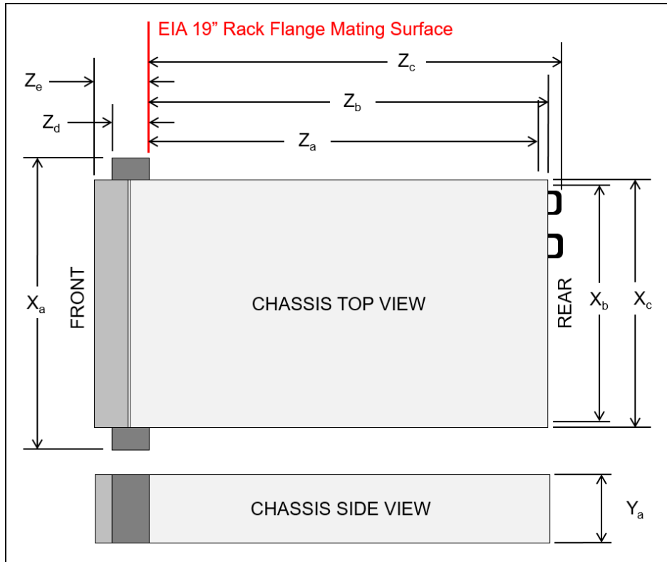
Figure 28. Server dimensions
